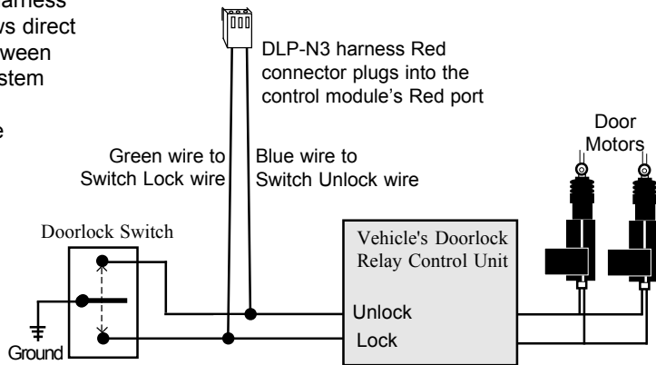
3 Wire Negative Doorlocks using the AL-100DP Control Unit outputs
