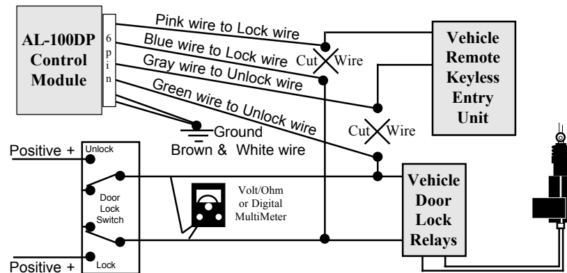
Type 1 Connection: Meter shows polarity change before the Lock and Unlock wires are cut. The doorlock relays and RKE unit are also separate.
